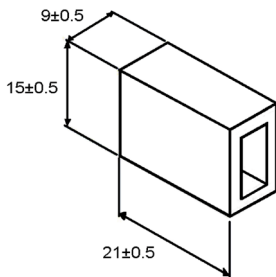
Base dimensions for Type B/Bf and I
