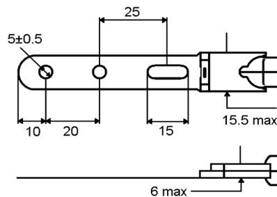
Metal clip dimension for Type J
